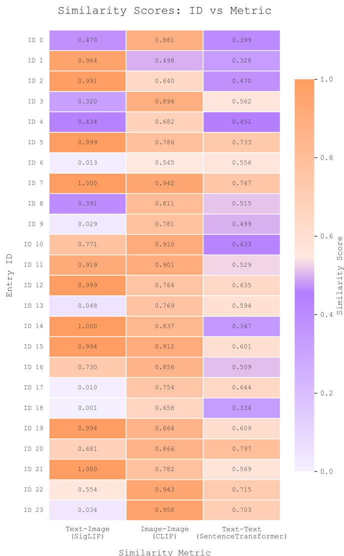
Figure 2: Heatmap of similarity scores across the 24 evaluated prompts. Rows correspond to entry IDs; columns show SigLIP (text-to-image), CLIP (image-to-image), and Sentence Transformers (text-to-text) metrics. Color scale ranges from low (purple, \approx 0.0 ) to high (orange, \approx 1.0 ) similarity. Darker purple regions indicate substantial deviation from the intended prompt semantics or visual structure.
